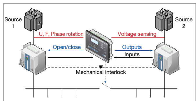
Circuit breaker (CB)
