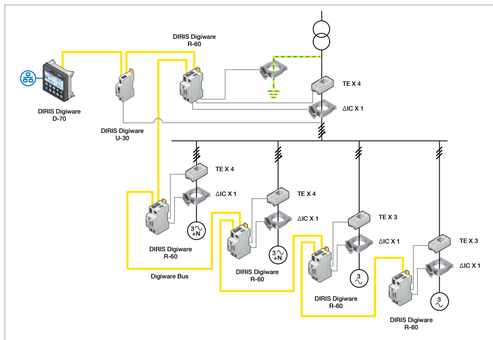
Fig. 15 – Example of an installation equipped with the DIRIS Digiware RCM system.
