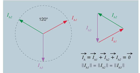
Fig. 10 – Example of a three-phase network with equal residual currents for each phase and phase-shifted by 120^\circ between them
