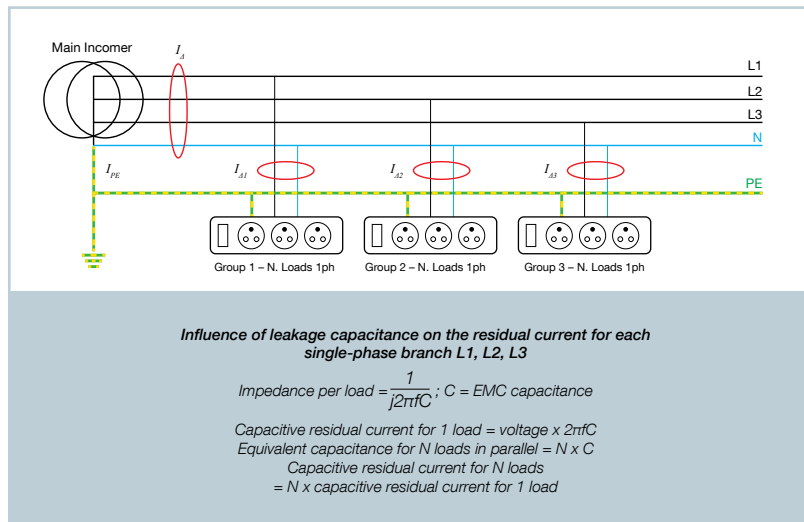
Fig. 11 – Increase in residual current based on the number of single-phase loads
