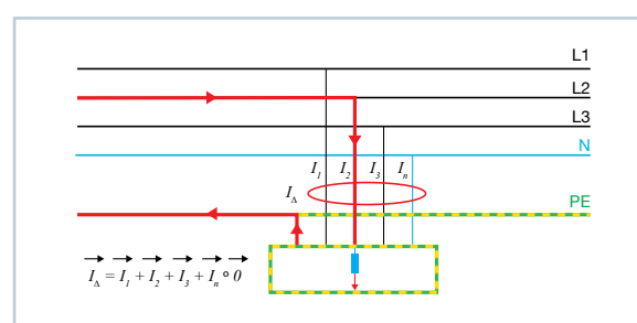
Fig.6 – TN-S system with residual current circulating through the PE
