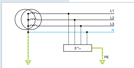
Fig. 1 – TT system
