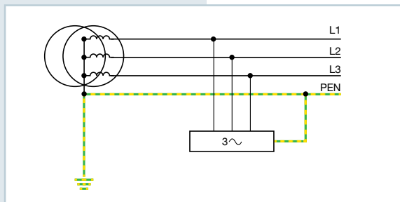
Fig. 2 – TN-C system
