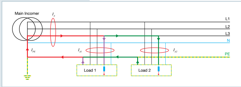
Fig. 8 – Relationship between the residual currents of the installation for a network and three-phase loads
