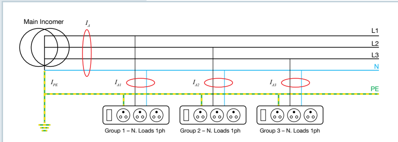
Fig. 10 – Example of a three-phase network with equal residual currents for each phase and phase-shifted by 120^\circ between them
