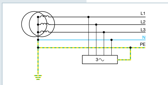
Fig.3 – TN-S system
