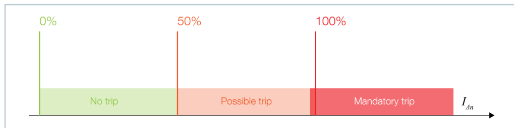
Fig. 14 – Trip thresholds of an RCD
