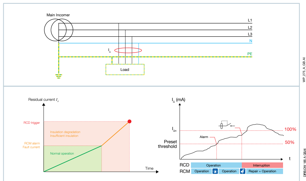
Fig. 7 – Temporal evolution of residual currents and difference between RCDs and RCMs
