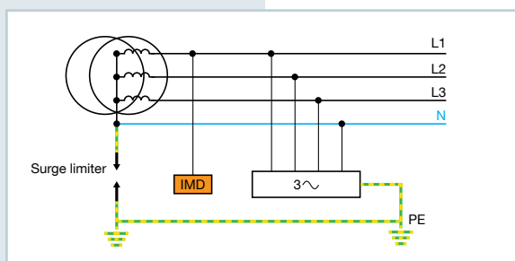
Fig.4 – IT system
