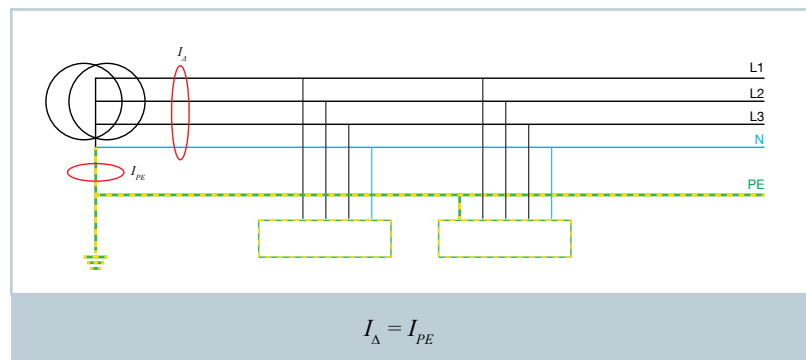
Fig. 12 – Measurement of the upstream PE conductor
