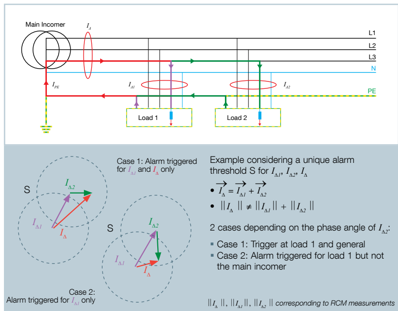
Fig. 9 – Example showing an alarm triggered at load level without triggering an alarm on the main incoher
