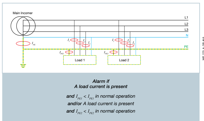
Fig. 13 – Measuring PE current at the loads
