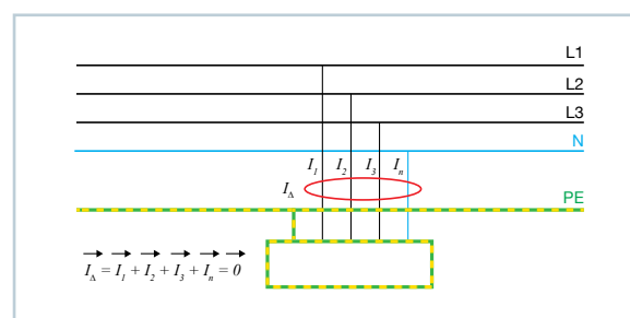
Fig.5 – TN-S system without residual current
